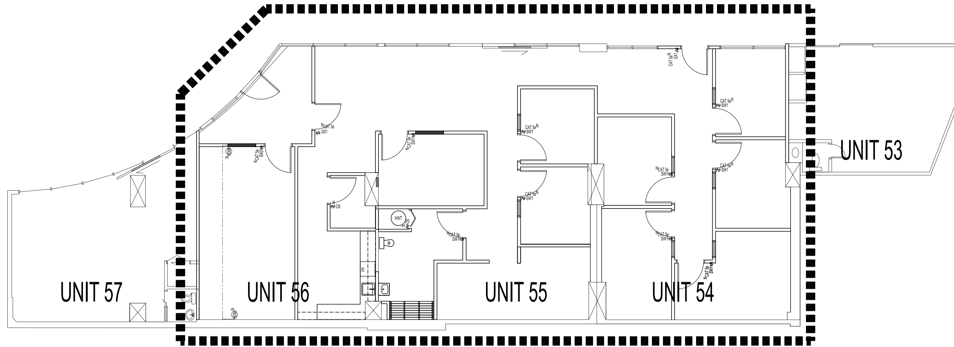
PARTIAL MEZZANINE PLAN - AREA OF WORK SCALE: 1/8"=1'-0"
