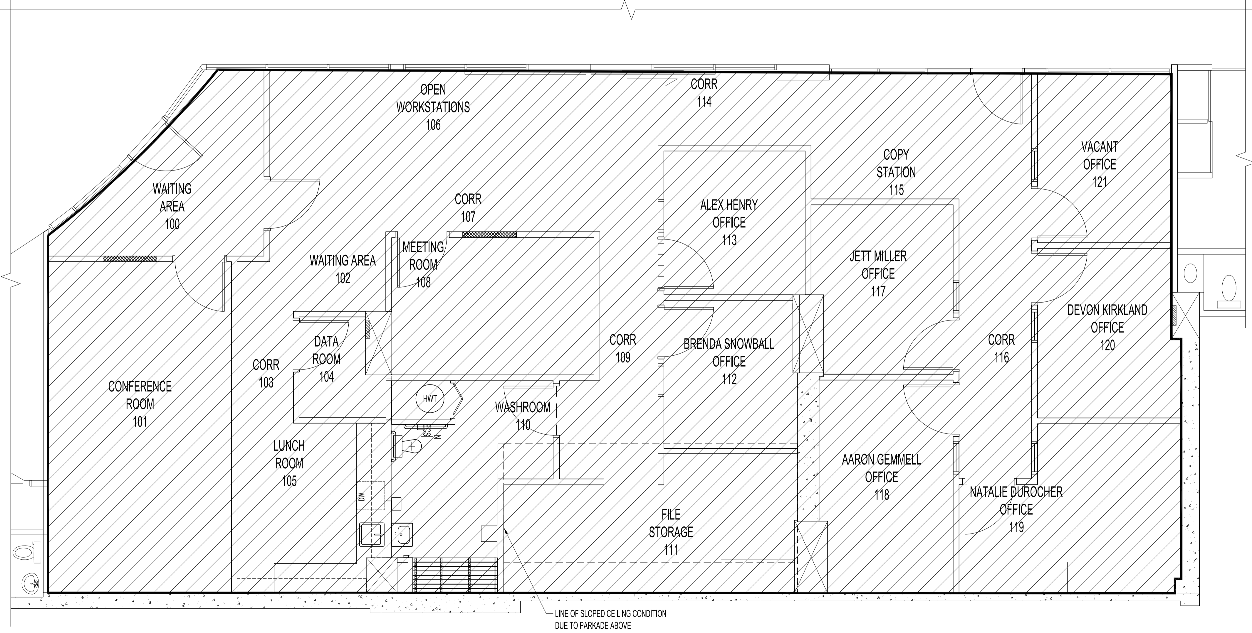
PARTIAL MEZZANINE PLAN - SCALE: 1/4"=1'-0"
